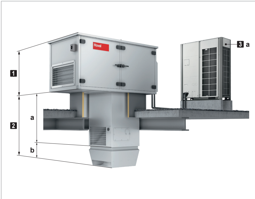
Image C1: Composants TopVent® SP
