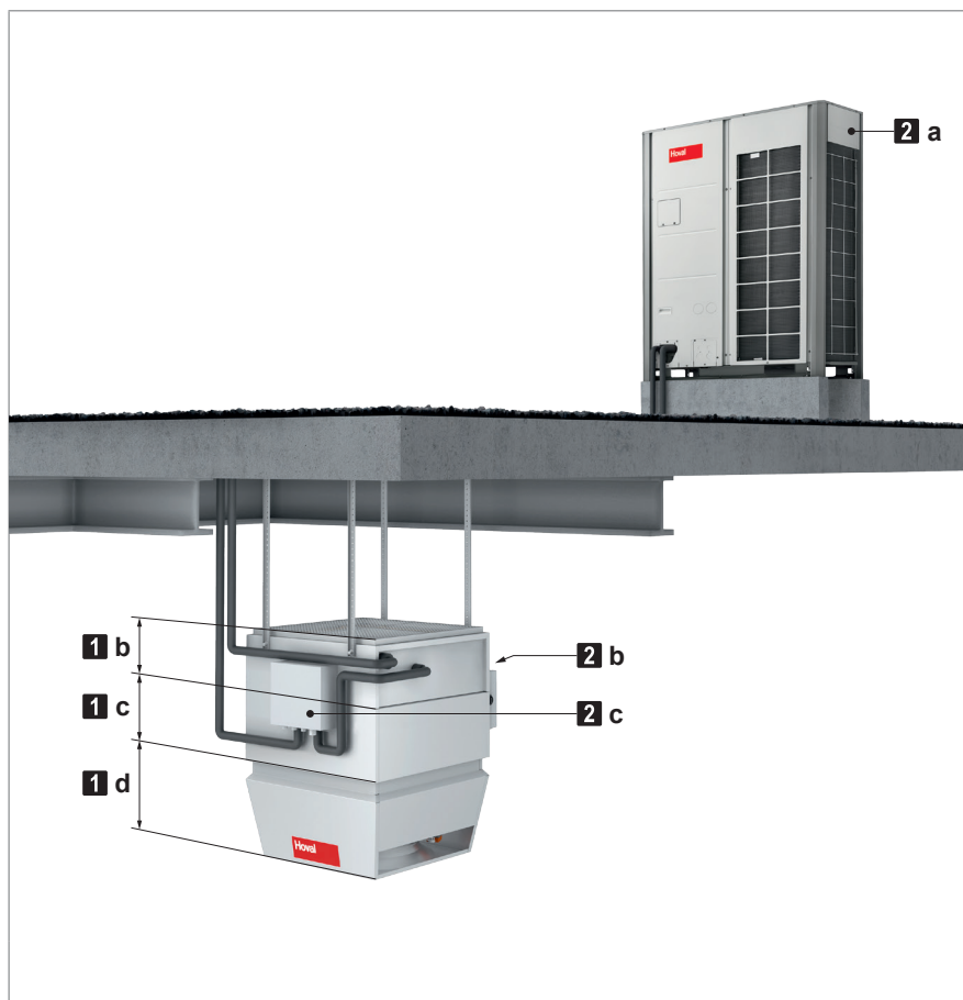
Fig. C1: Composants TopVent® TPH
